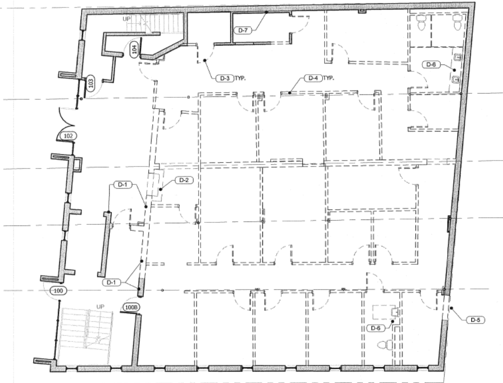
1 1st FLOOR PLAN 1/8" = 1'-0"
